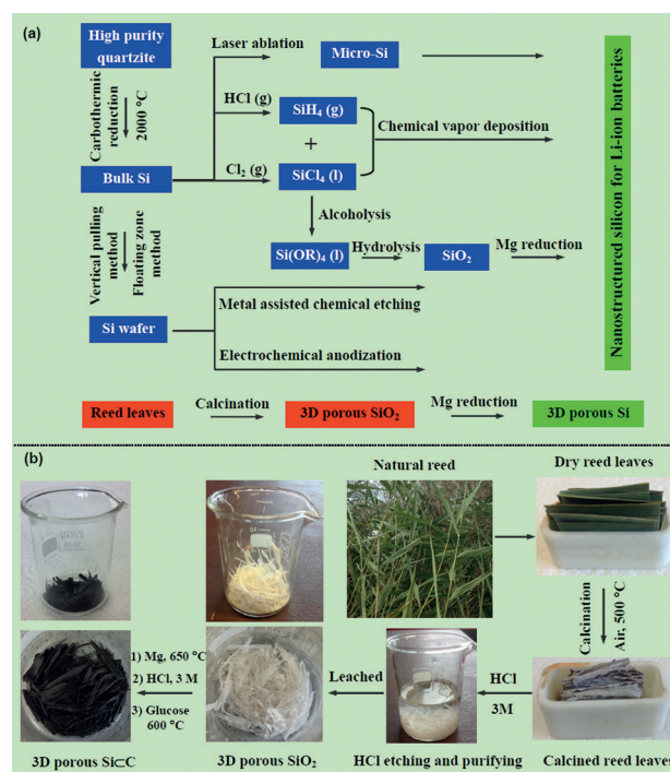
Scheme 1. a) Flow chart showing conventional synthesis routes of nano-Si for Li-ion battery anodes, and along with of our sustainable and low-cost synthesis route from natural reed leaves. b) Detailed flow chart of the process for 3D porous SiC anode from natural reed leaves to the 3D porous \text{SiO}_2 precursor and finally the 3D porous SiC anode.
